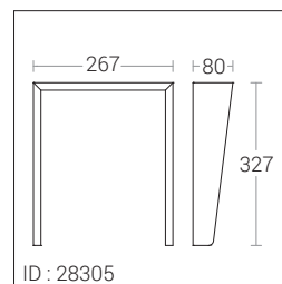
Anti Glare Shield ID : 28305
